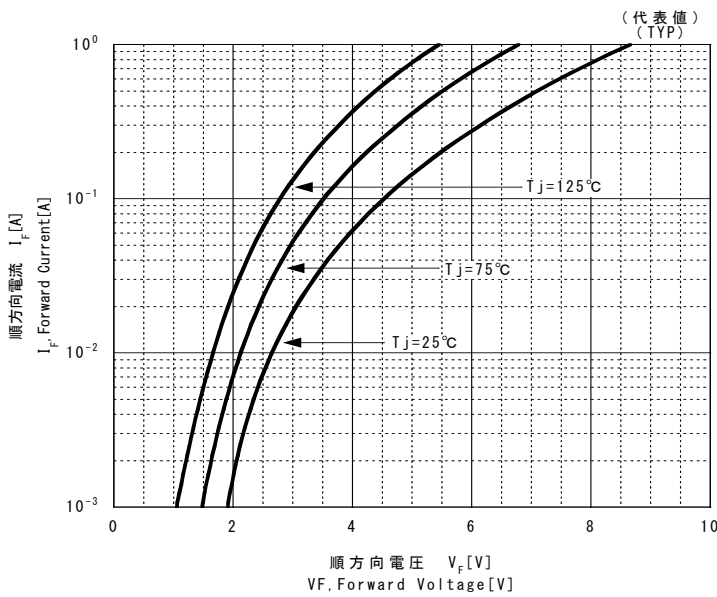
FORWARD CHARACTERISTICS
